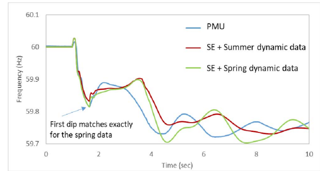
Figure 8. Frequency results at a different 500 kV bus to show seasonal dynamic data impacts on the first dip
