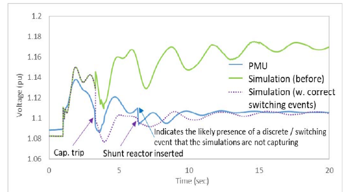
Figure 9. Voltage comparisons at a 500 kV bus before and after accounting for reactive power switching events
