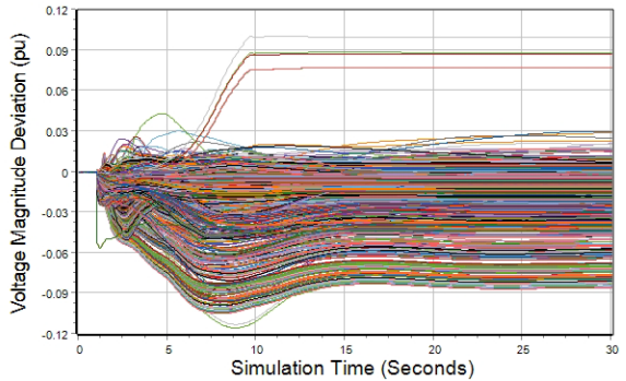
Figure 10: WECC Voltage Deviation
