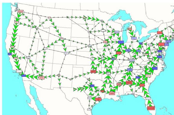
Figure 4: 82K Grid Inter-Area Power Flows
