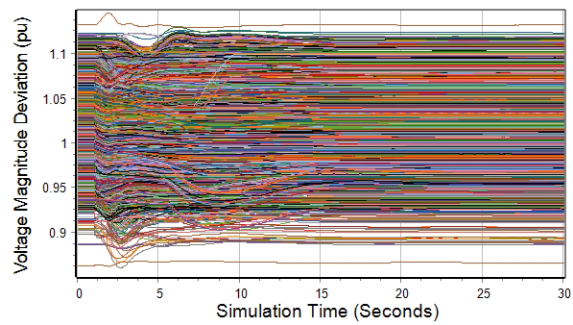
Figure 9: Actual WECC Voltage Magnitude Response
