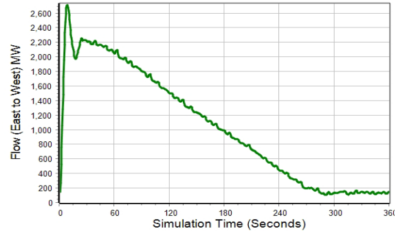
Figure 11: Interface Flow for Simulation with AGC
