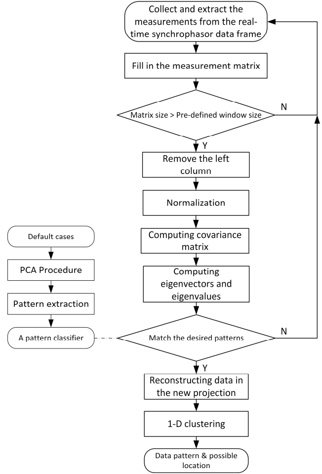
Fig. 4 Flowchart of the PCA-based scheme
