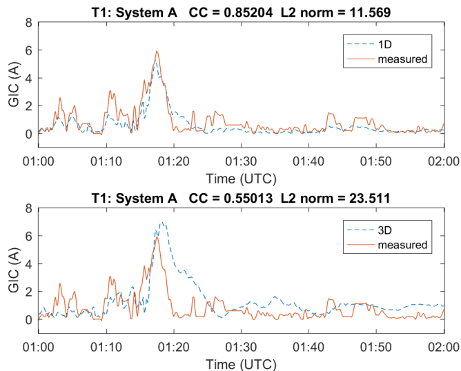
Figure 5 Zoomed in Simulated and Measured GICs at T1
