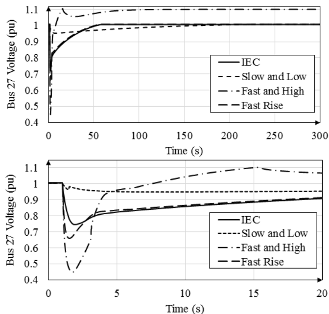
Fig. 7. Comparisons of the system response to 40% field intensities
