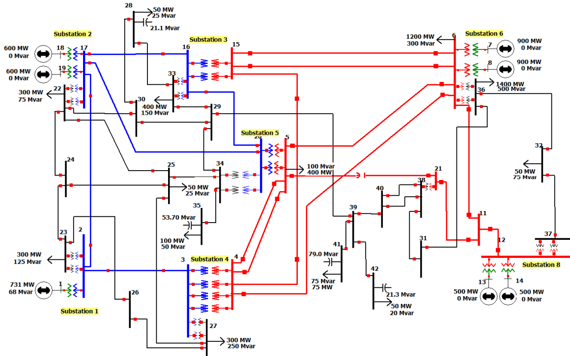
Fig. 1. 42 bus test case
