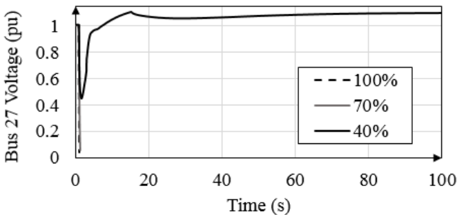
Fig. 5. System response to the fast and high rising geoelectric field
