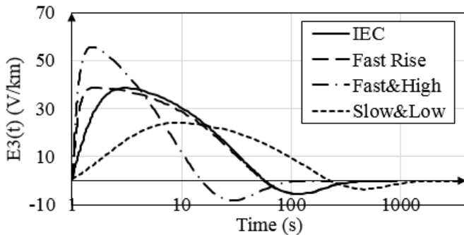
Fig. 2. Geoelectric fields used for simulations, 100% scaling
