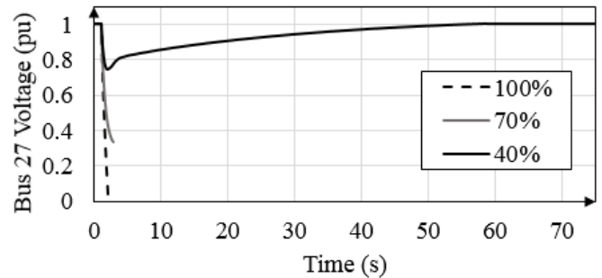
Fig. 3. System response to the IEC reference geoelectric field
