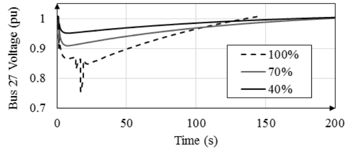
Fig. 6. System response to the slow and low rising geoelectric field
