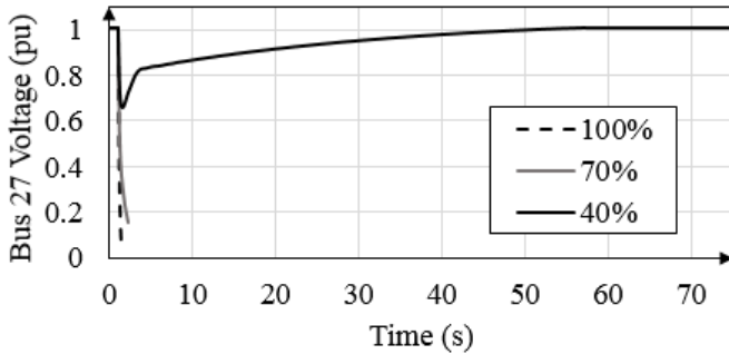
Fig. 4. System response to the fast rising geoelectric field
