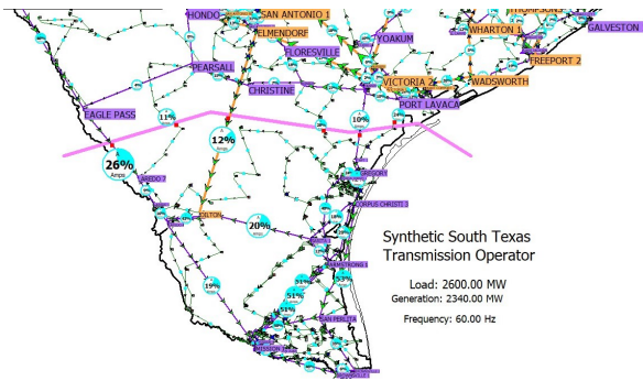
Fig. 7. The target area (i.e. Southern Texas) in the synthetic Texas grid
