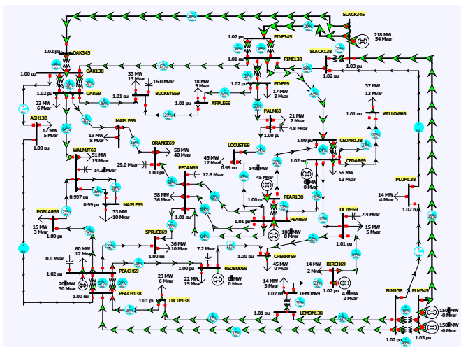
Figure 2: 37-Bus System Oneline
