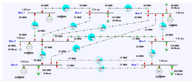
Figure 1: Seven Bus System Oneline
