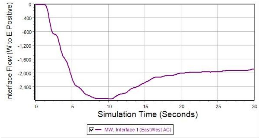
Figure 3.6 Interface Flow MW (West to East Positive) Over 30 Seconds
