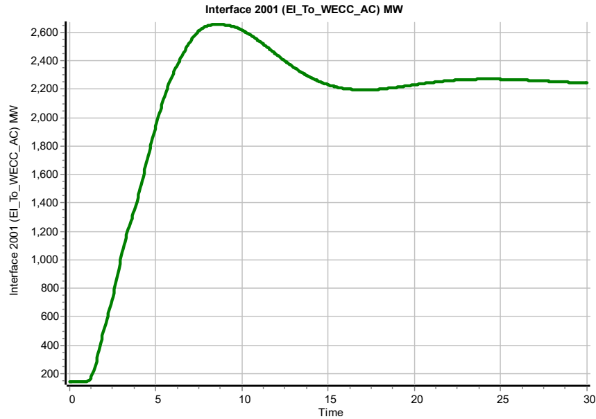
Figure 3.1 MW Flows on the EI-WI Interface
