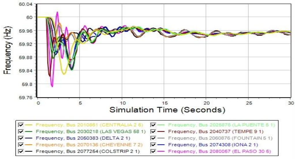
Figure 3.7 Frequency Response at Ten Buses in the West Over 30 Seconds
