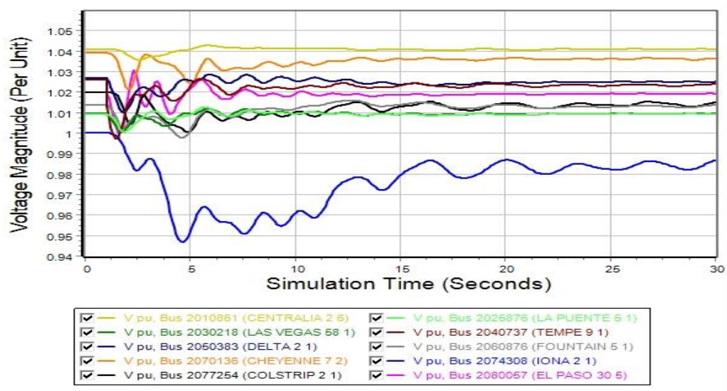
Figure 3.8 Voltage Magnitude Response at Ten Buses in the West Over 30 Seconds
