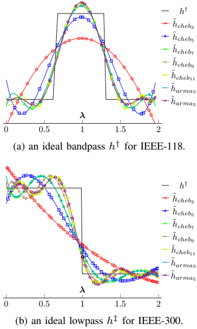
Fig. 4. Empirical frequency responses of CHEB and ARMA GFs when approximating ideal filters h^\dagger and h^{\ddagger} applied on IEEE 118- and 300-bus test systems, respectively. Compared to CHEB, ARMA better approximates the desired filter for the same K (e.g. \tilde{h}_{cheb3} vs \tilde{h}_{arma3} ) and it requires a lower K for the same level of approximation (e.g. \tilde{h}_{cheb11} vs \tilde{h}_{arma5} ).
