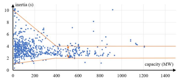
Fig. 3. Dependence of machine inertia on generator capacity for coal units
