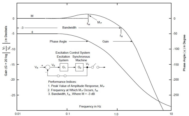
Fig. 12. Typical closed-loop frequency responses of an excitation control system with the synchronous machine open-circuited [17]
