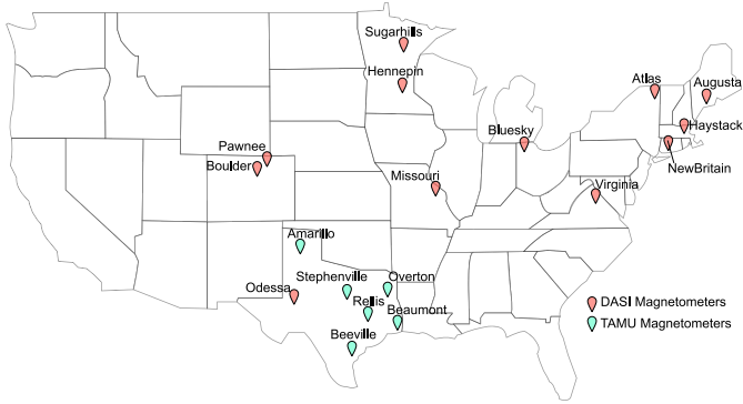
Fig. 2. Magnetometer locations within the DASI and TAMU magnetometer networks presented with red and green icons, respectively.
