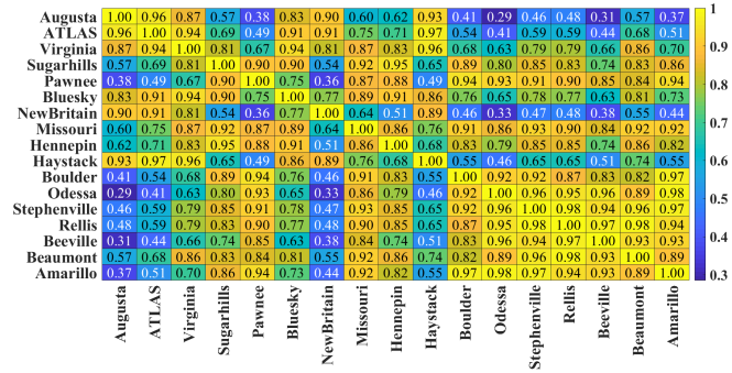
(b) Correlation of B_Y on the storm commencement day (Nov. 3).
