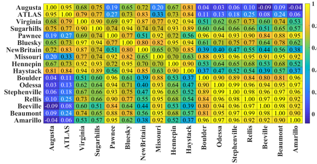
(a) Correlation of B_Y on the typical pre-event day (Nov. 2).
