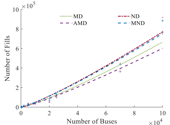
Fig. 1. The number of fills vs. the number of buses.
