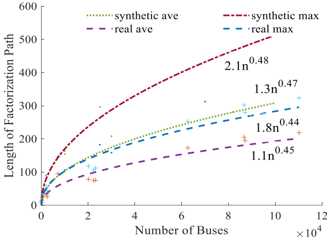
Fig. 3. The average and the longest factorization path vs. the number of buses.
