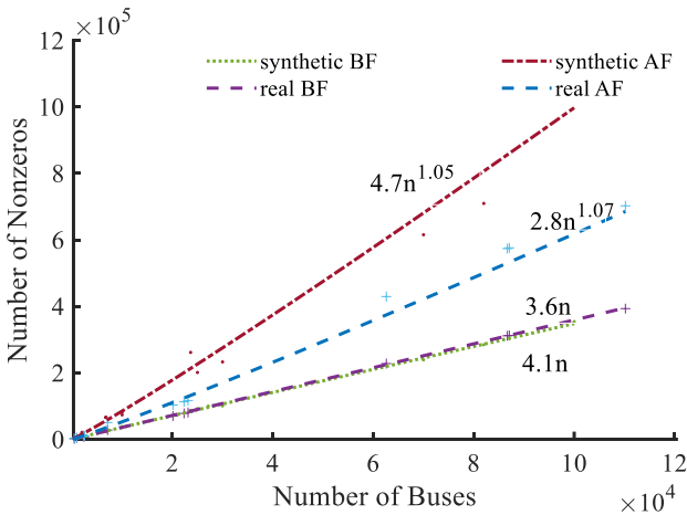
Fig. 4. The number of nonzeros B/A factorization vs. the number of buses.
