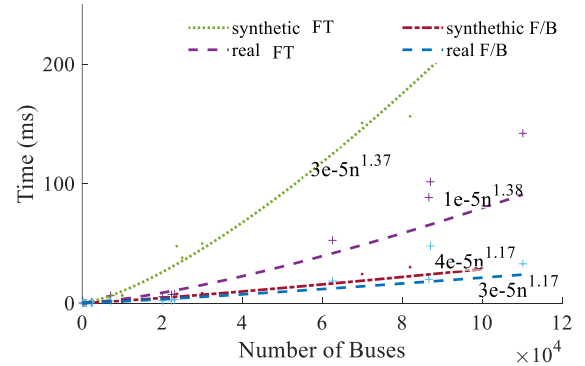
Fig. 2. The Factorization time and F/B time vs. the number of buses.
