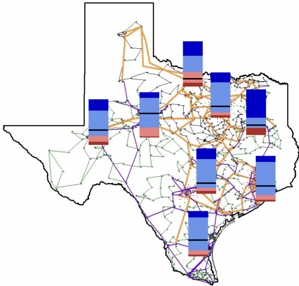
Fig. 4: VRR GDVs at the simulation hour of 3:00 AM.
