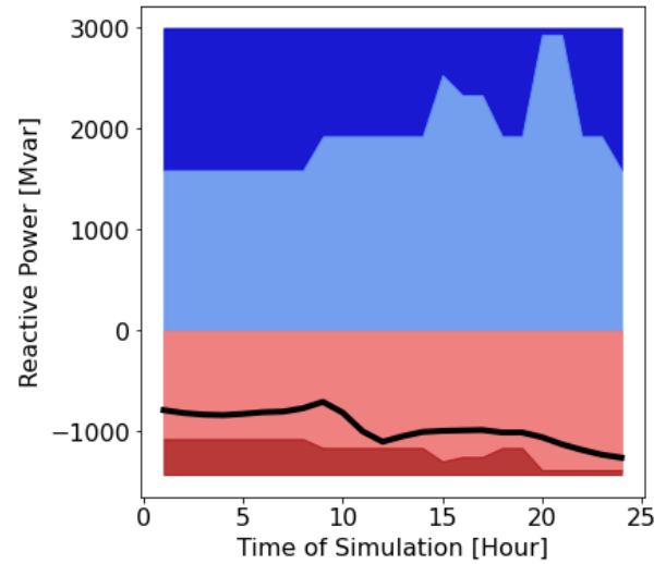
(b) North area VRR chart.
