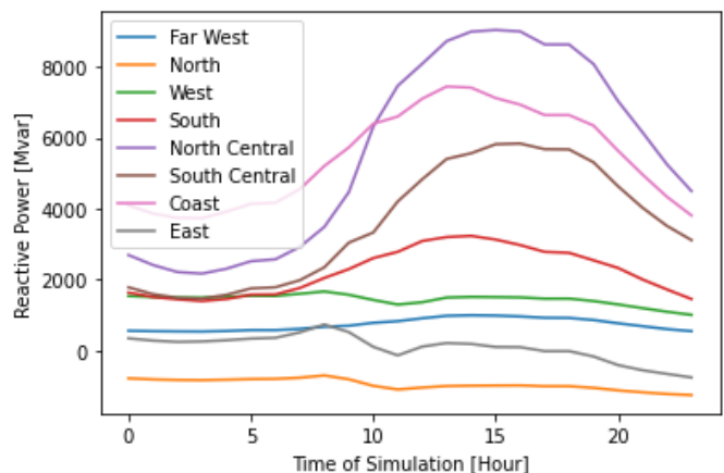
Fig. 2: Reactive power dispatch levels within each area of the case over the 24-hour simulation window.
