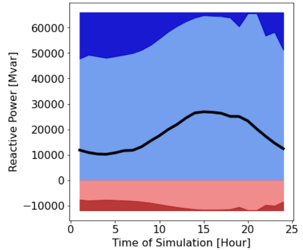
(a) System-wide VRR chart.
