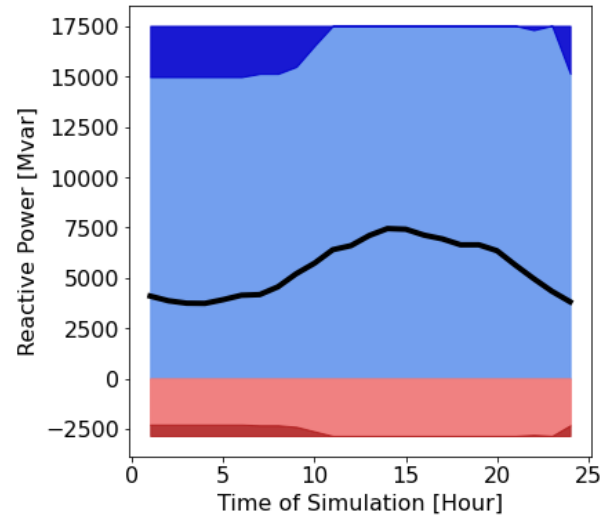
(c) Coast area VRR chart.
