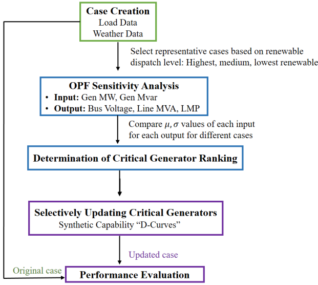
Fig. 1: Flow chart of selectively updating generator capability curves.
