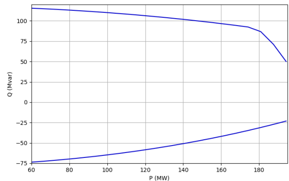
Fig. 4: An example of generator capability curve: Bus 1053 in 2000 bus case.
