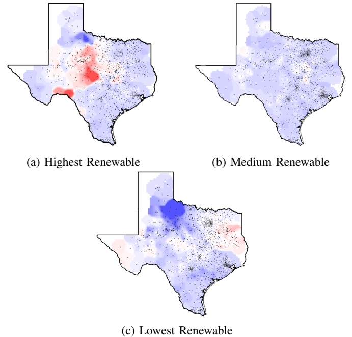
Fig. 2: Bus voltage magnitudes for the highest, medium, lowest renewable 2000 bus cases.
