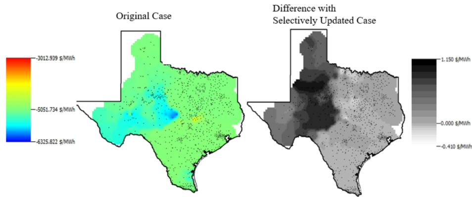
Fig. 5: Bus LMPs in OPF solution for original 2,000 bus base case (left). Difference contours with comparison to base for selectively updated case (right).
