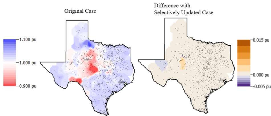
Fig. 6: Bus voltage magnitudes in OPF solution for original 2,000 bus base case (left). Difference contours with comparison to base for selectively updated case (right).
