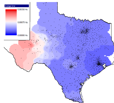
Figure 6: Spatial Variation in Bus Average Frequency Error
