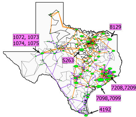
Figure 1: Texas 2000 Bus System Oneline
