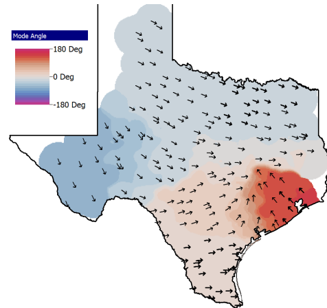
Figure 12: Visualization of 0.64 Hz Mode from a Forced Oscillation
