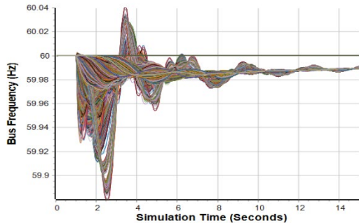
Figure 14: EI Frequency Response for a New England Generator Outage
