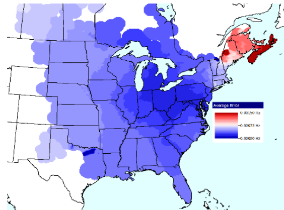
Figure 18: Spatial Variation in Bus Average Frequency Error
