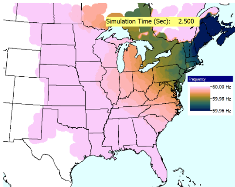
Figure 15: Spatial Frequency for the Figure 14 Scenario at 2.5 Seconds
