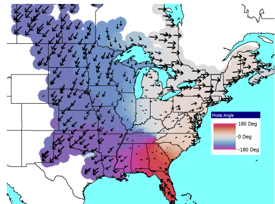
Figure 17: NEng Scenario, 0.27 Hz Mode Shape, 21.3% Damping
