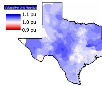
Fig. 8: Voltage contour visualization for one-time point for the year 2030.
