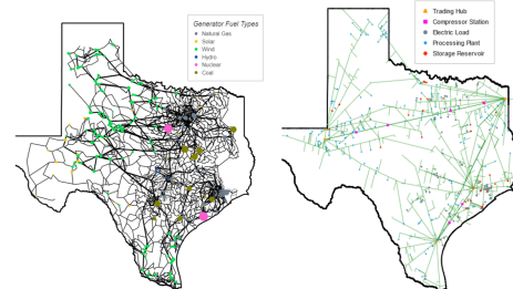
Fig. 3: Combined transmission and gas network for the Texas-7k case.
