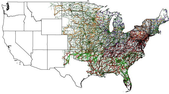
Fig. 2: ACTIVSg70k: 70,000 bus power grid network on the footprint of Eastern United States.
