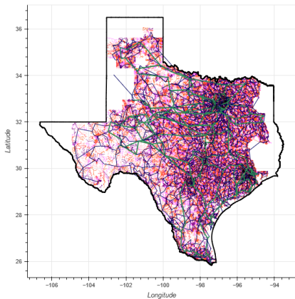
Fig. 4: Combined transmission and distribution network for the Texas-7k case.
