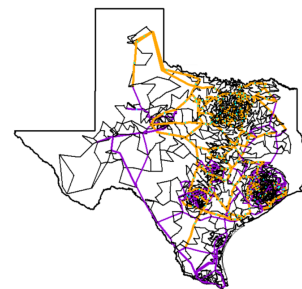
Fig. 1: ACTIVSg2000: 2000 bus power grid network on the footprint of Texas
