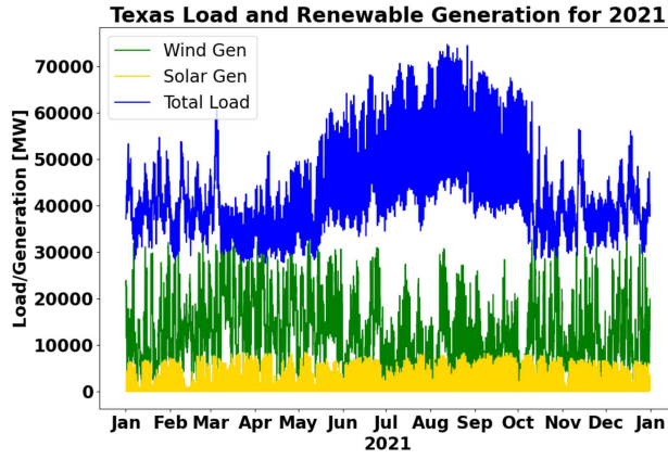
Fig. 4: Texas Load and Generation 2021
