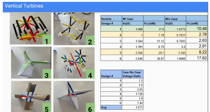
Fig. 7. Wind turbines with the vertical axis and comparison of their power outputs
