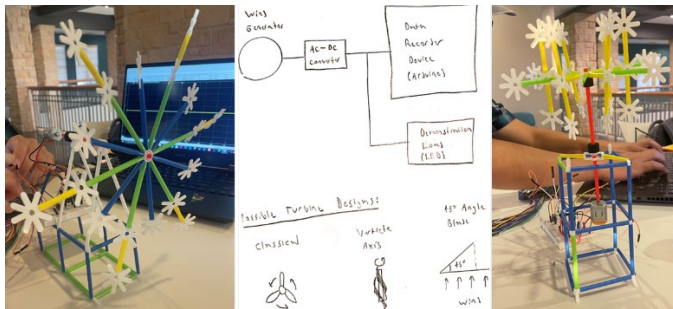
Fig. 5. The initial design sketch (middle), and first horizontal axis (left) and vertical axis (right) wind turbines
