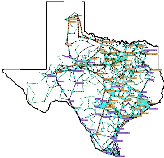
Fig. 3. One-line Diagram for the ACTIVSg2000 Test Case
