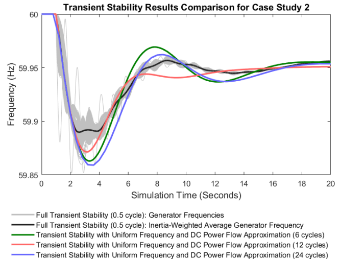
Fig. 4. Frequency Stability Results Comparison for Case Study 2
