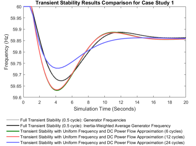
Fig. 2. Frequency Stability Results Comparison for Case Study 1
