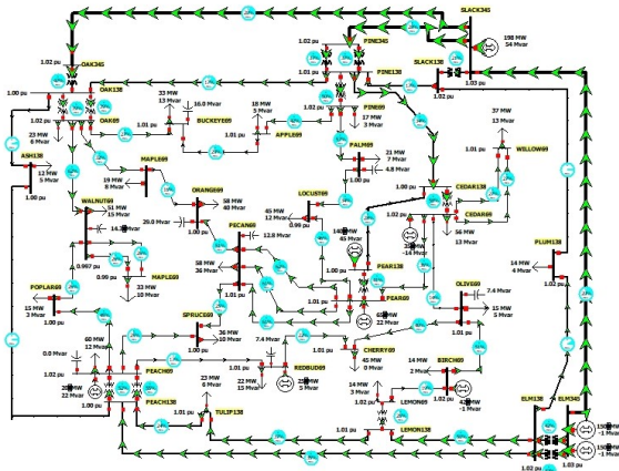
Fig. 1. One-line Diagram for the 37-bus Test Case
